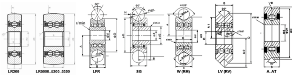
LFR Series track rollers bearings
