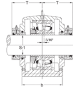
TACONITE SEAL OPTION
